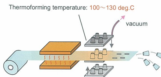
Thermoforming process
